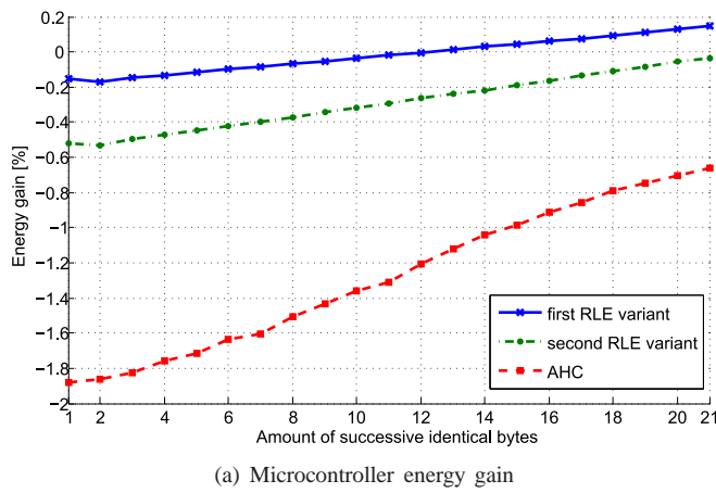
Fig. 4. Resulting best case energy gains
