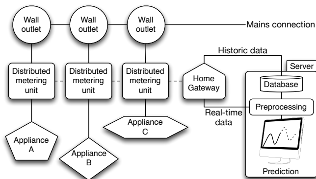
Fig. 1. System architecture of the proposed demo
